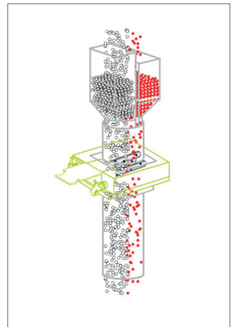
The SAFEMAG inline magnet is used in standing or slow-moving material columns.
